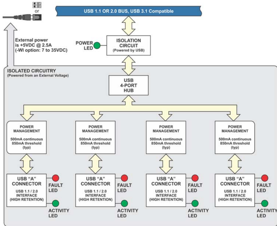
BLOCK DIAGRAM
